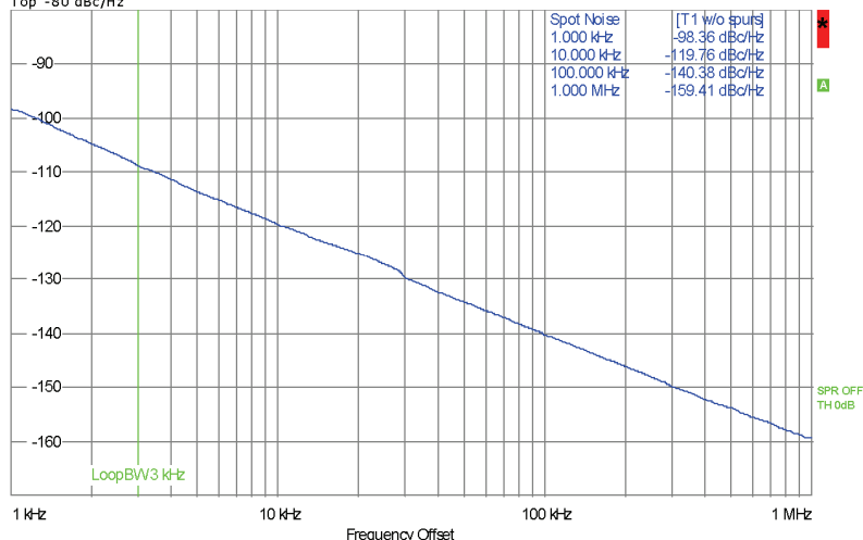
Phase Noise [dBc/Hz] RF Atten 10 dB manual Top -80 dBc/Hz
