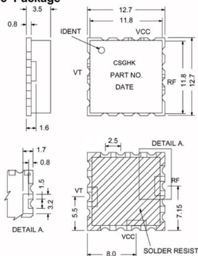
SK605 Package
